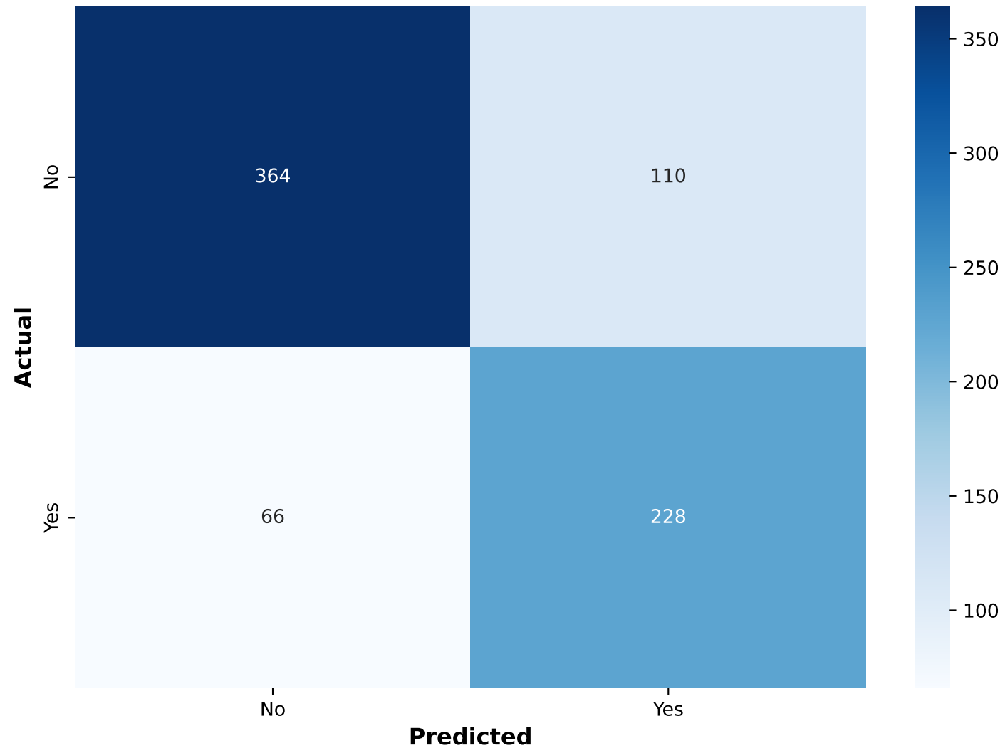
CatBoost - Test Set
