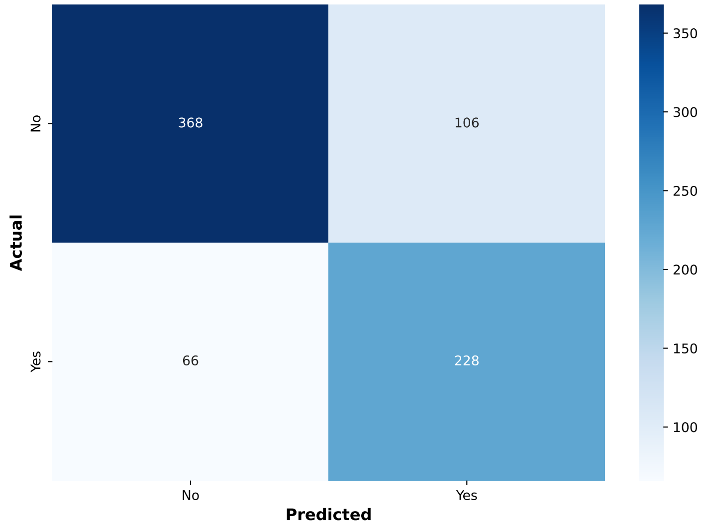
GBM - Test Set
