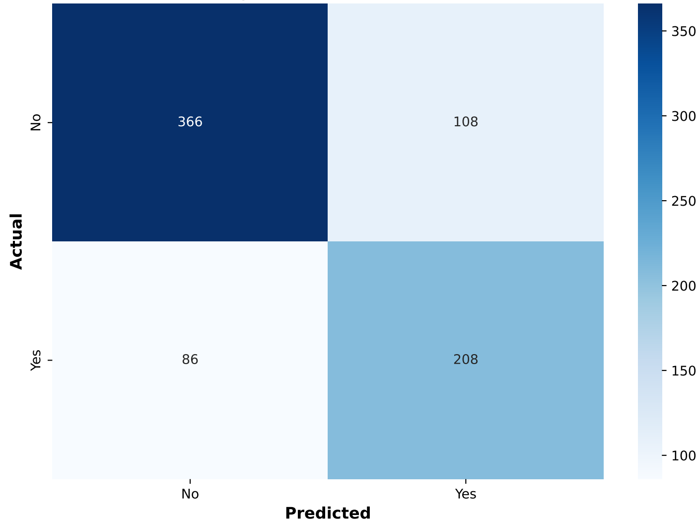
LightGBM - Test Set
