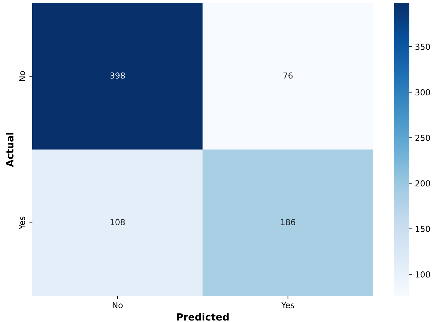
NeuralNetwork - Test Set
