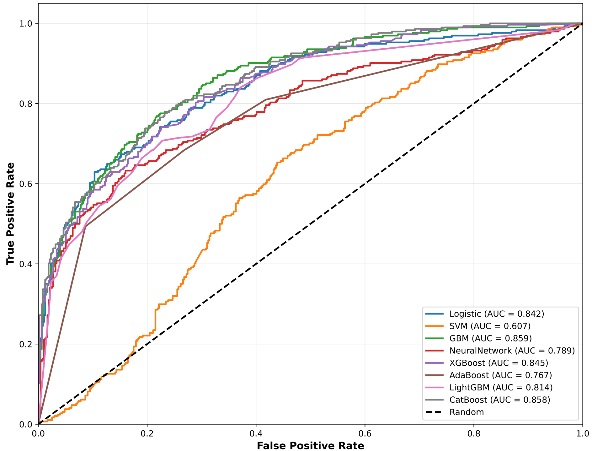
ROC Curve - Test Set
