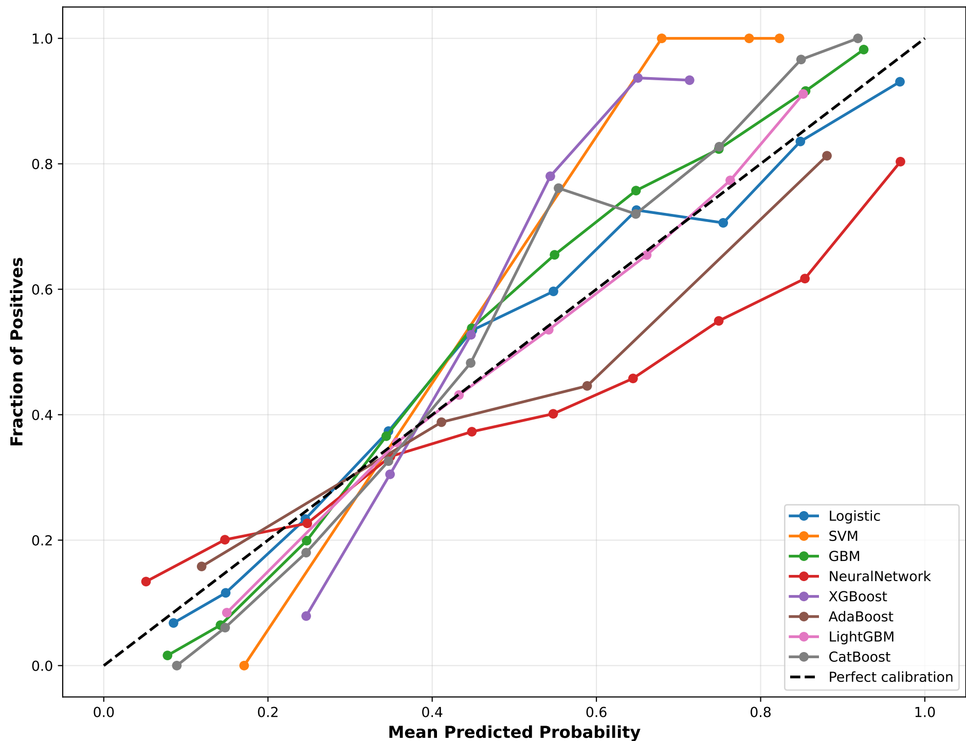
Calibration Curve - Train Set
