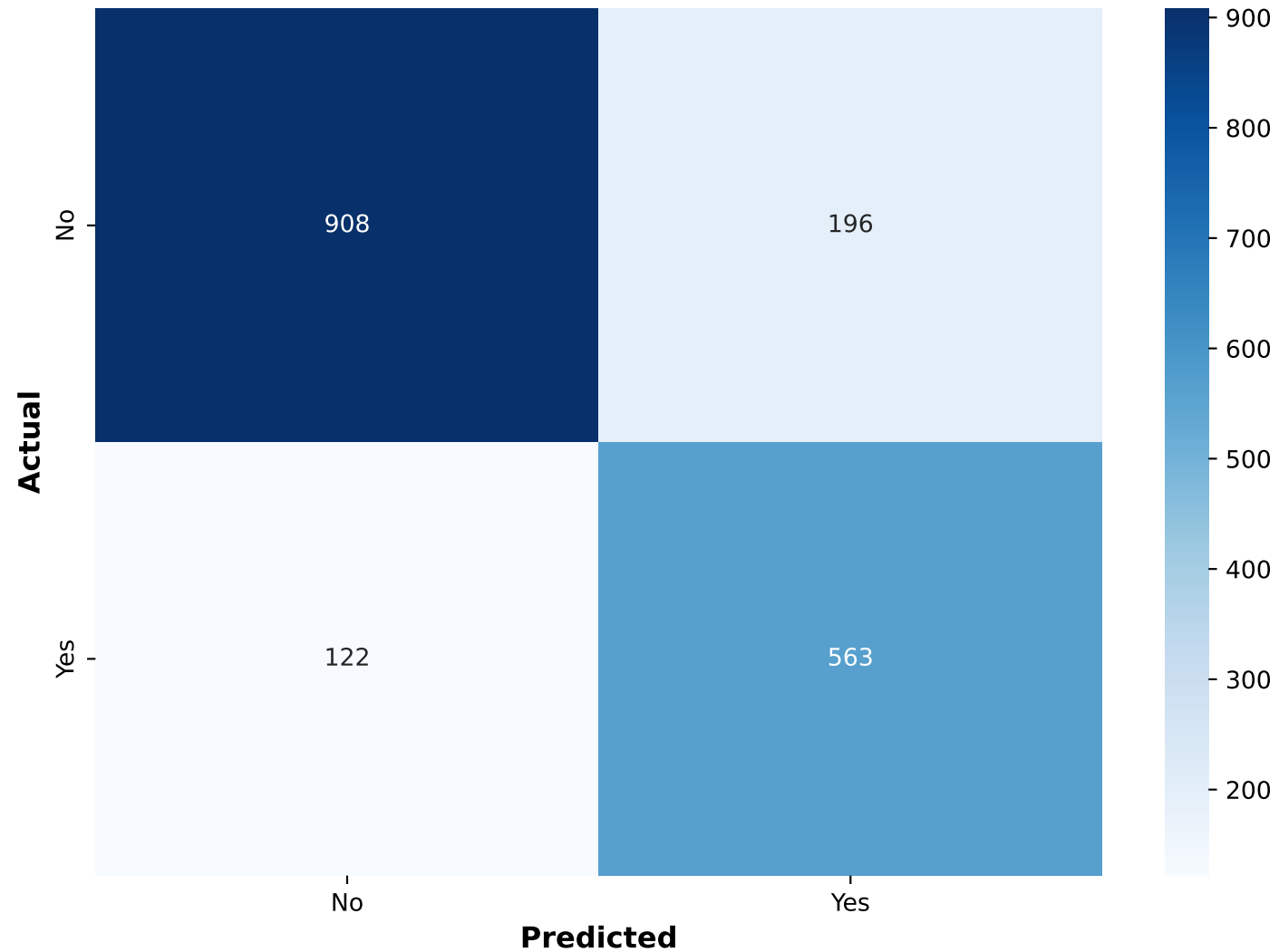
CatBoost - Train Set
