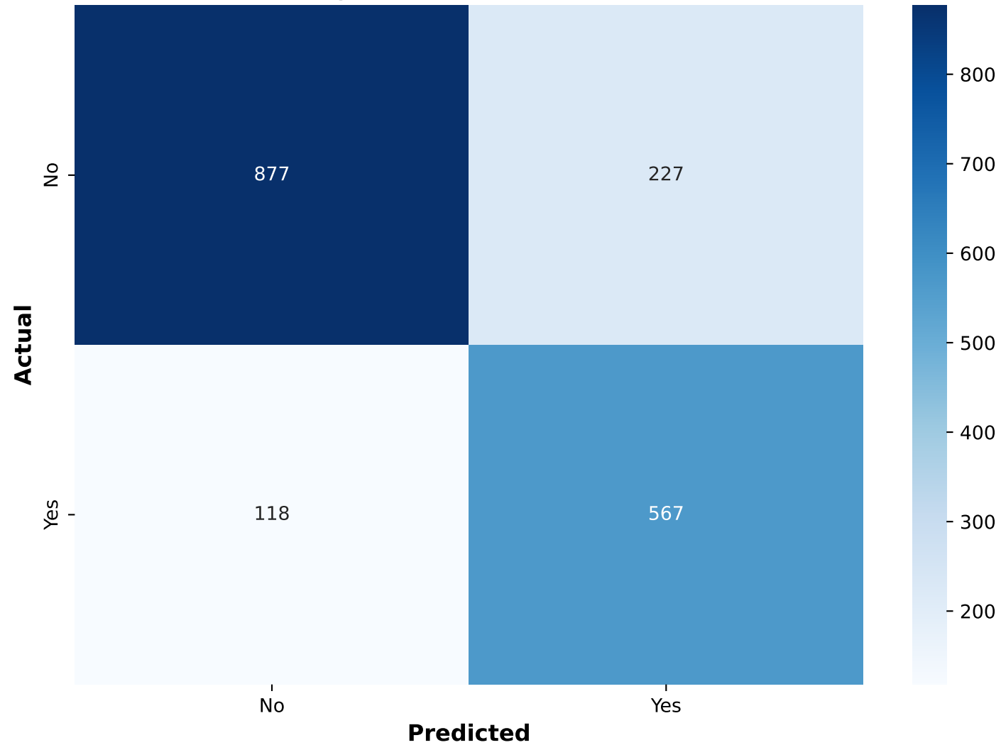
LightGBM - Train Set
