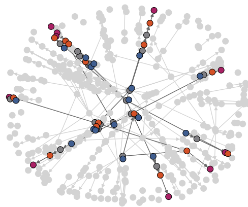
MolSculptor
