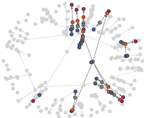
EvoSynth (Contrastive)
