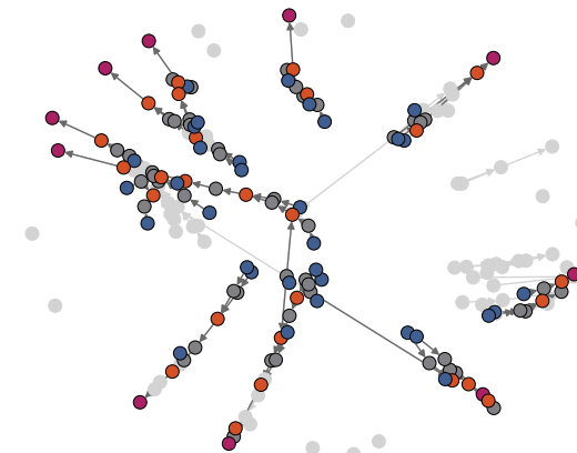
CMD-GEN
