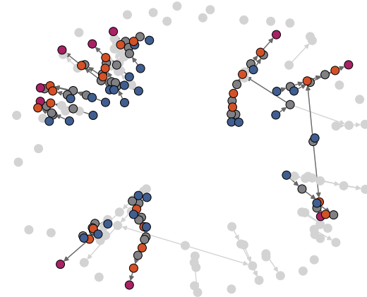
CMD-GEN
