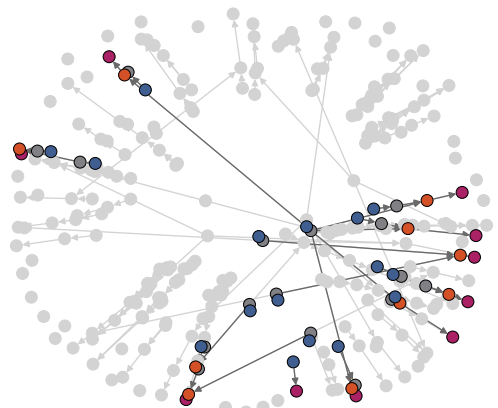
EvoSynth (Predictor)
