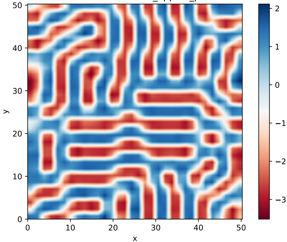
Generated Pattern: u_{\text{approx\_pinn}}
