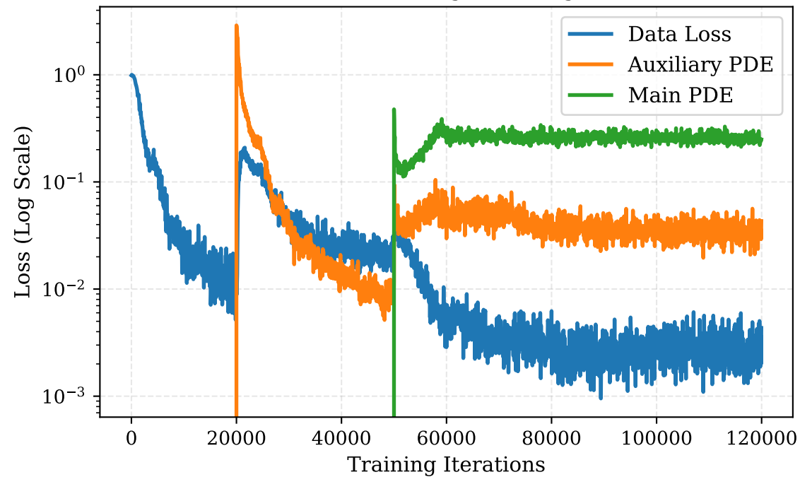
Loss Convergence (Log)
