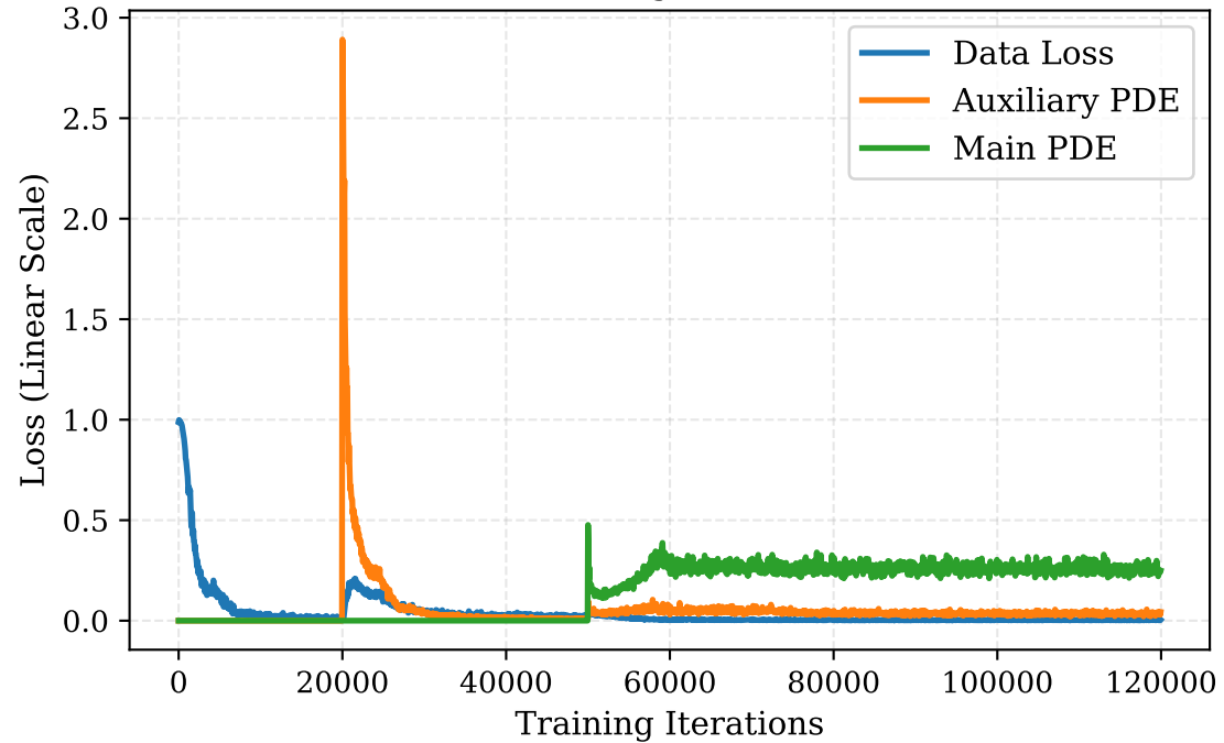
Loss Convergence (Linear)
