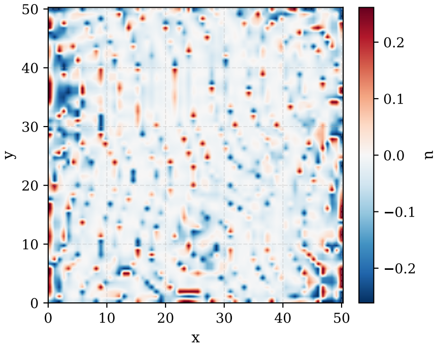
Relative Error
