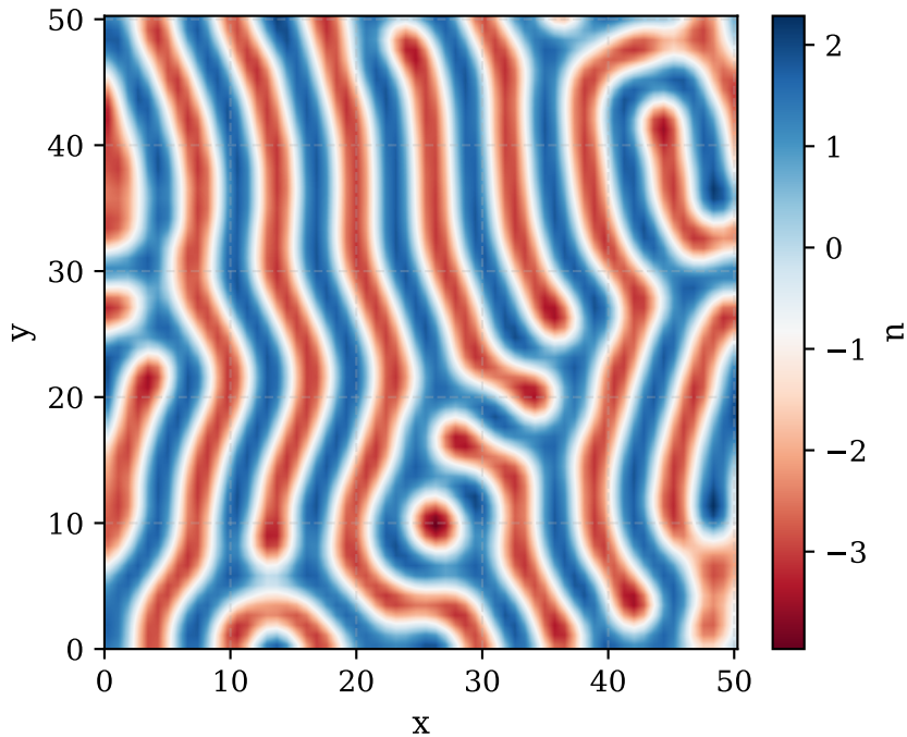
PINN Prediction
