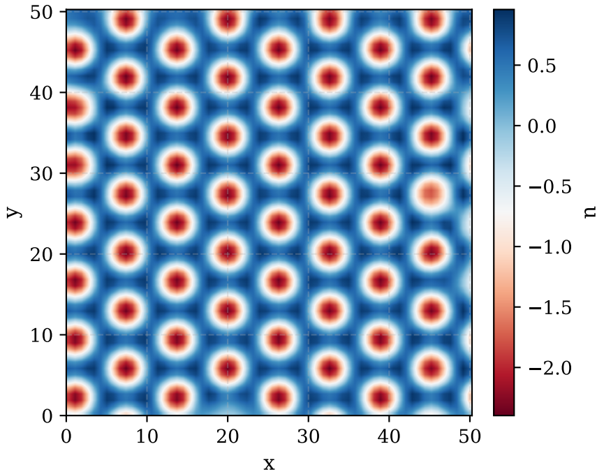
PINN Prediction
