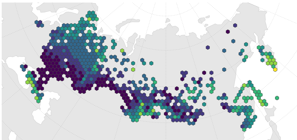
(a) Mean discharge ( \text{mm d}^{-1} )
