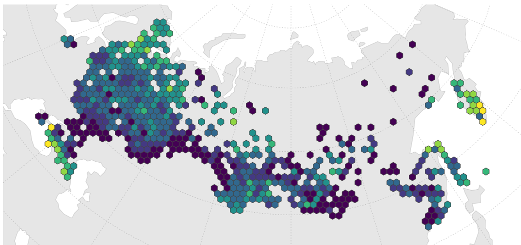
(b) Low flow: 5th percentile (95% exceedance; \text{mm d}^{-1} )
