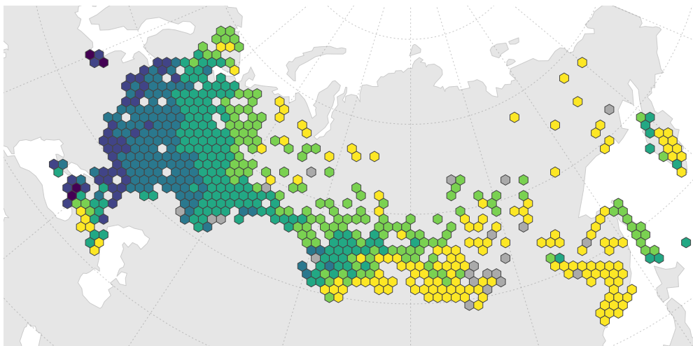
(a) Mean half-flow date (day of hydrological year)
