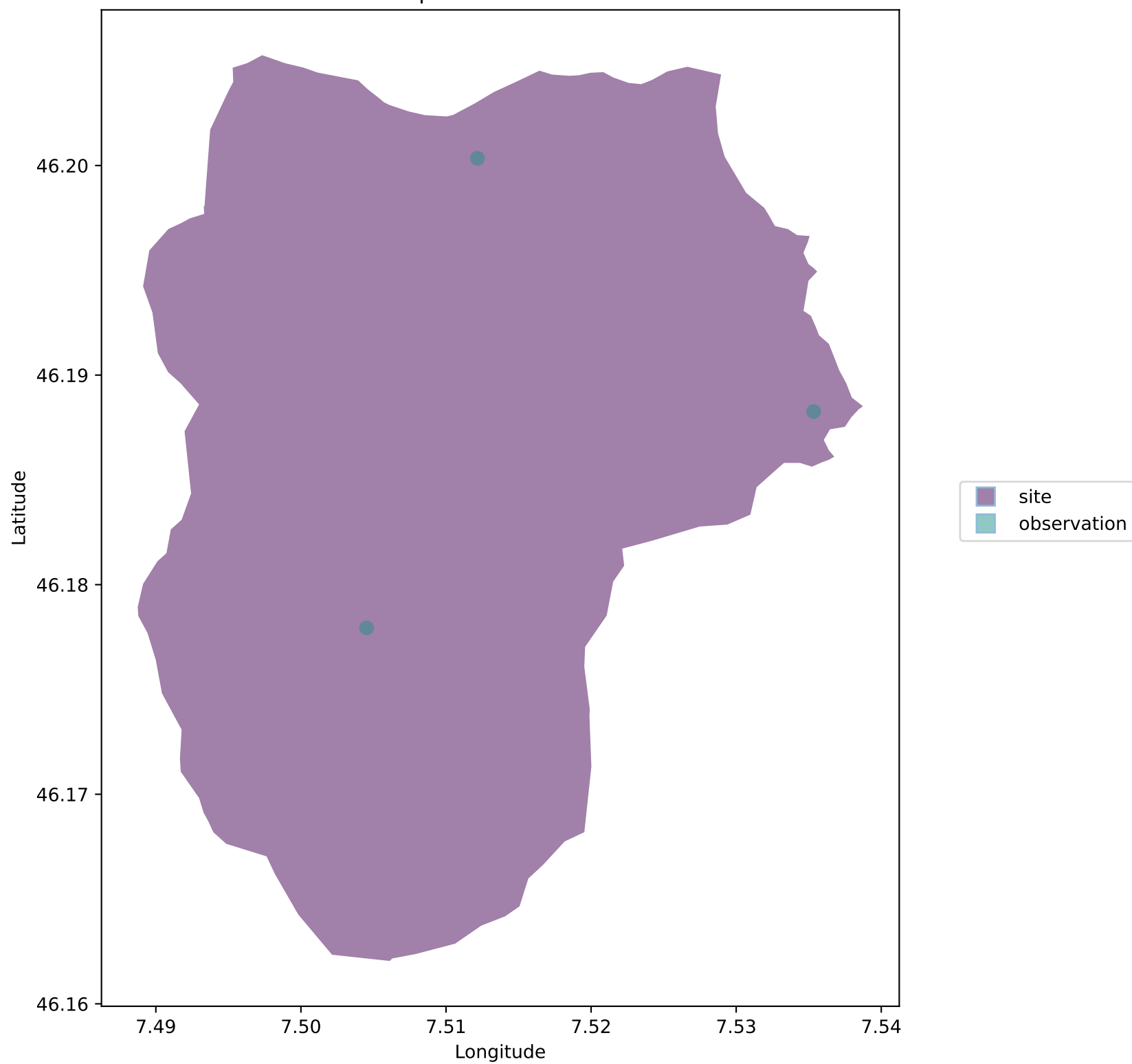
Multiple GeoDataFrames
