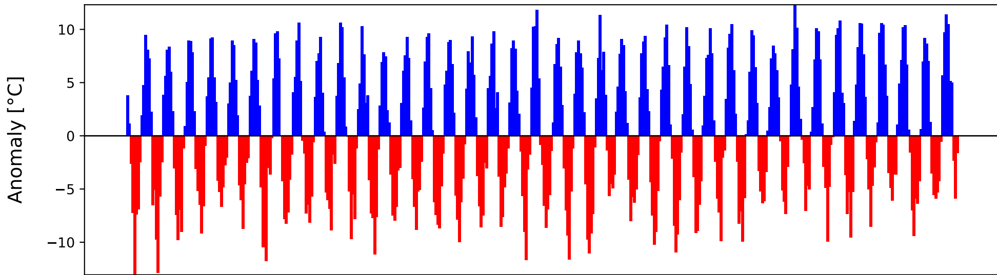
Monthly Air Temperature Anomalies [ ^{\circ}\text{C} ]
