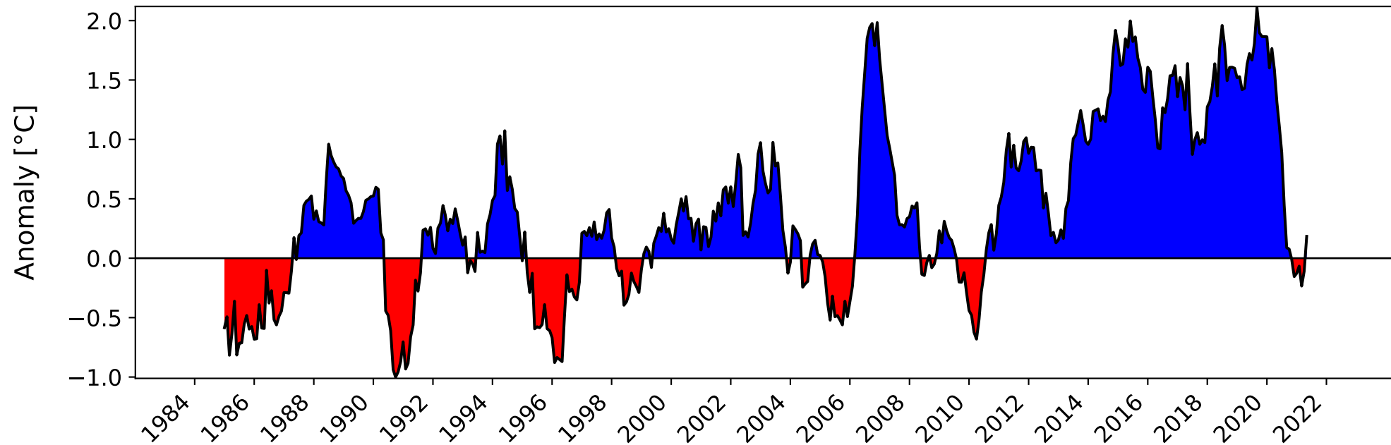
12-Month Rolling Average Air Temperature Anomalies [ ^{\circ}\text{C} ]
