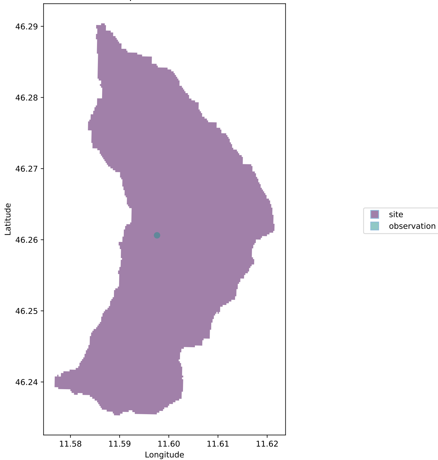
Multiple GeoDataFrames
