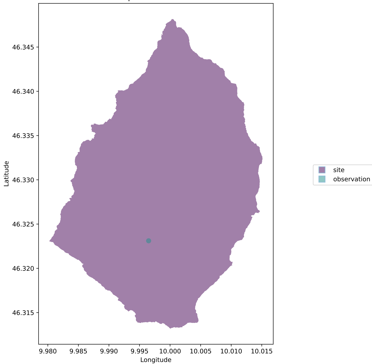
Multiple GeoDataFrames
