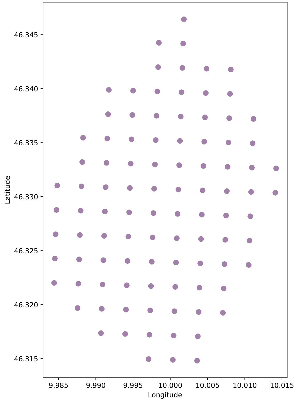
Multiple GeoDataFrames
