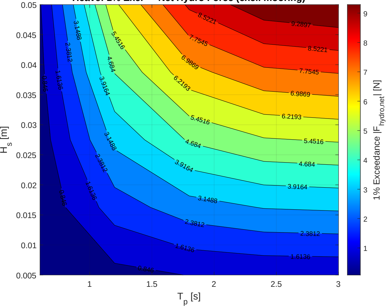
Heave: 1% Exc. — Net Hydro Force (excl. mooring)
