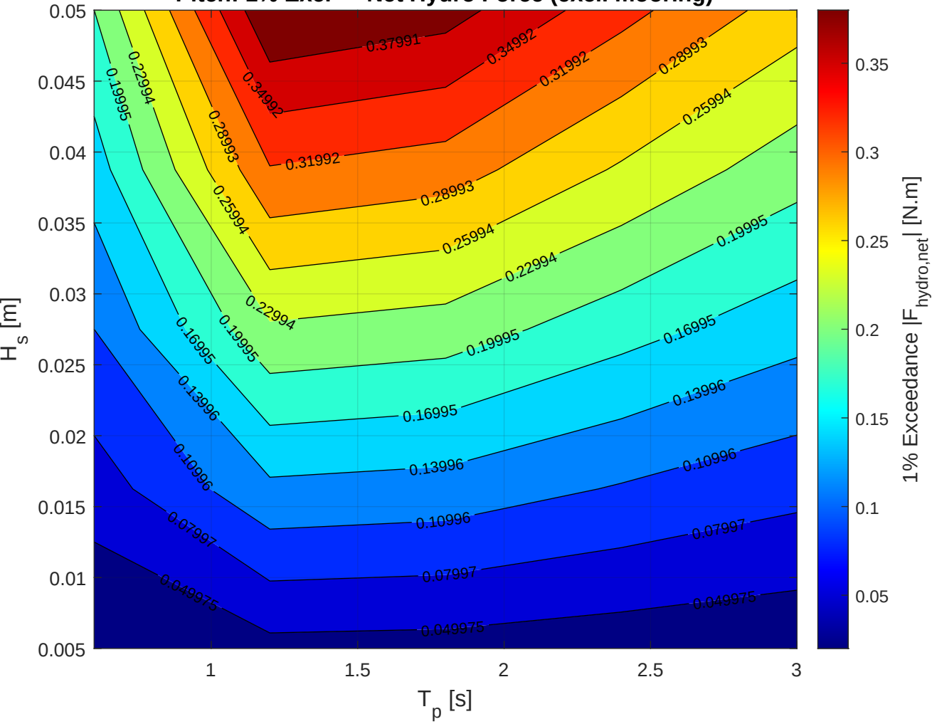
Pitch: 1% Exc. — Net Hydro Force (excl. mooring)
