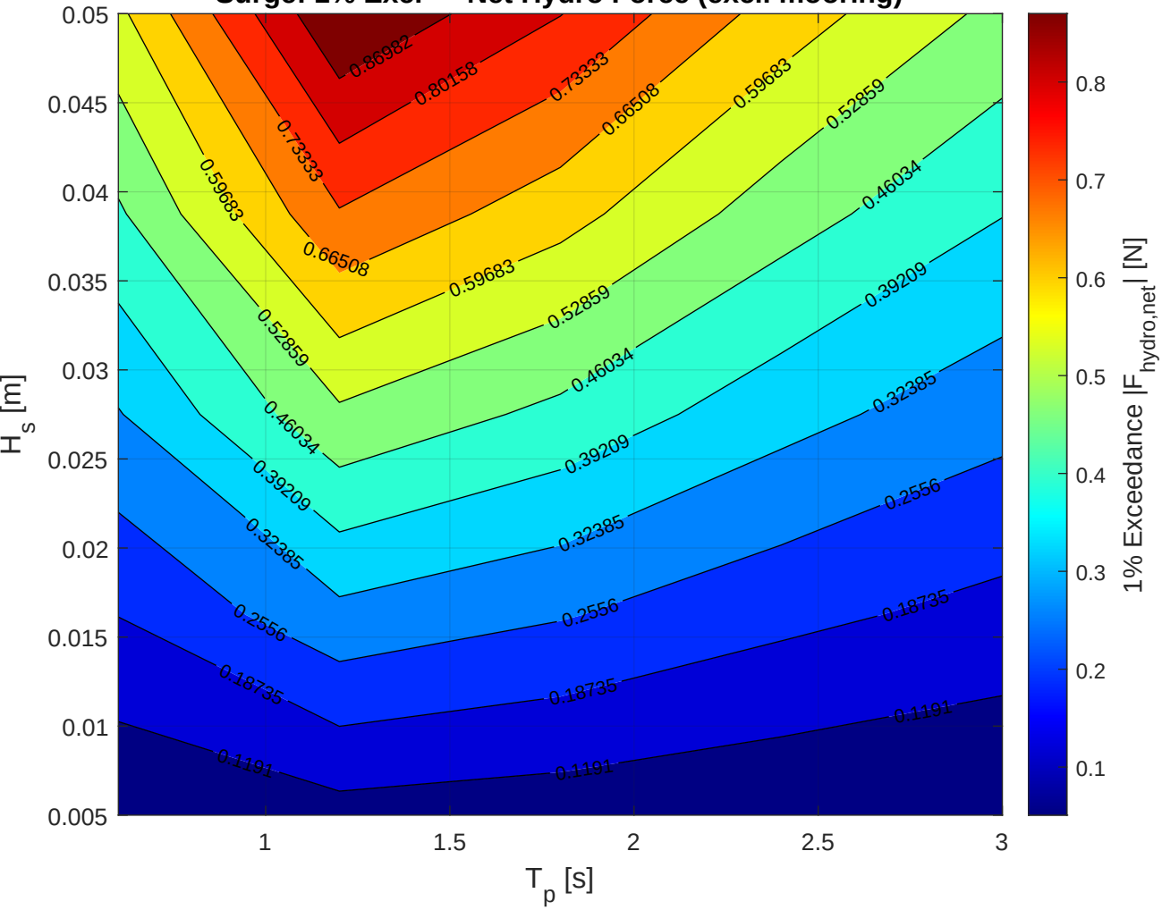
Surge: 1% Exc. — Net Hydro Force (excl. mooring)
