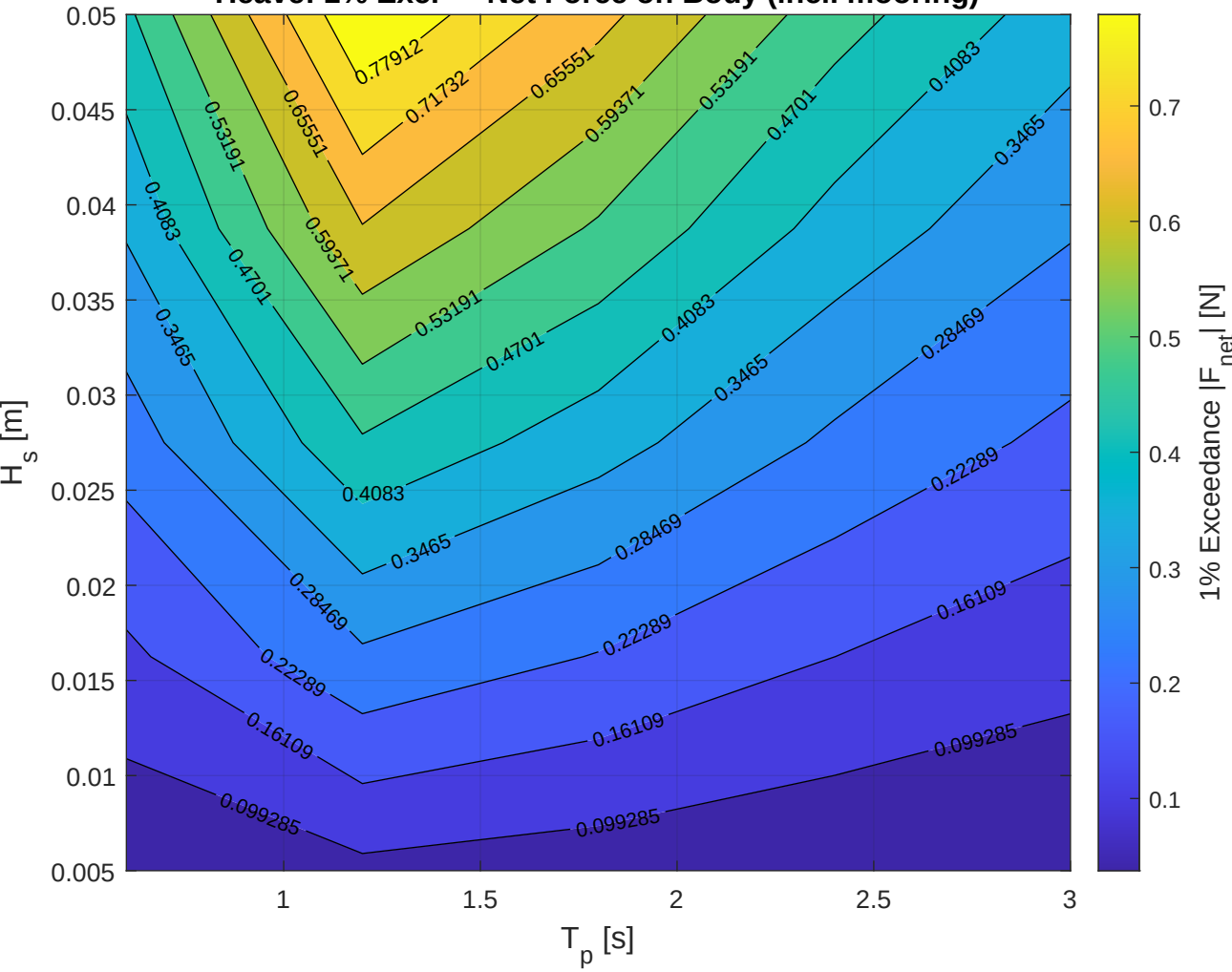
Heave: 1% Exc. — Net Force on Body (incl. mooring)
