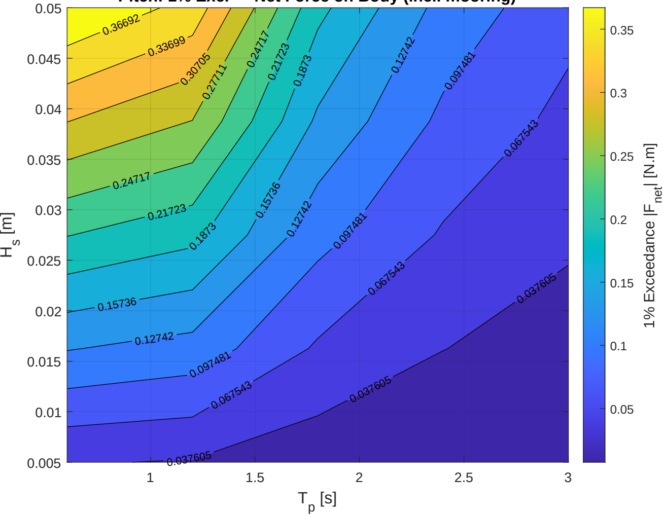
Pitch: 1% Exc. — Net Force on Body (incl. mooring)
