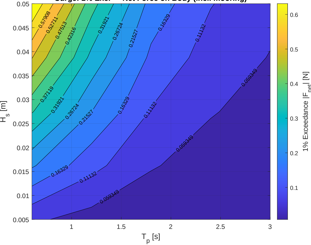
Surge: 1% Exc. — Net Force on Body (incl. mooring)
