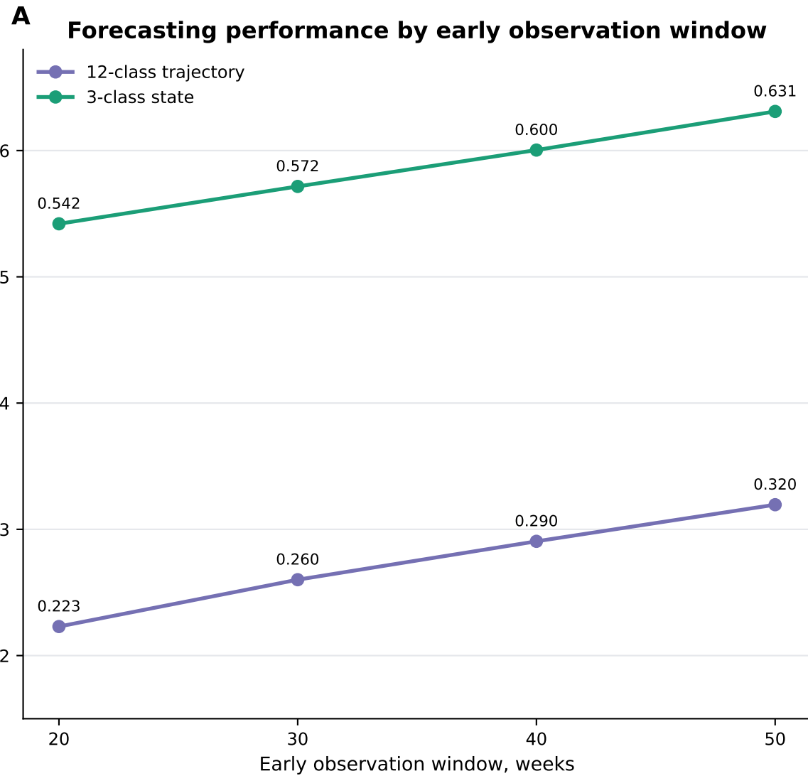
Figure 3. Early prediction improves with temporal dynamics and context
