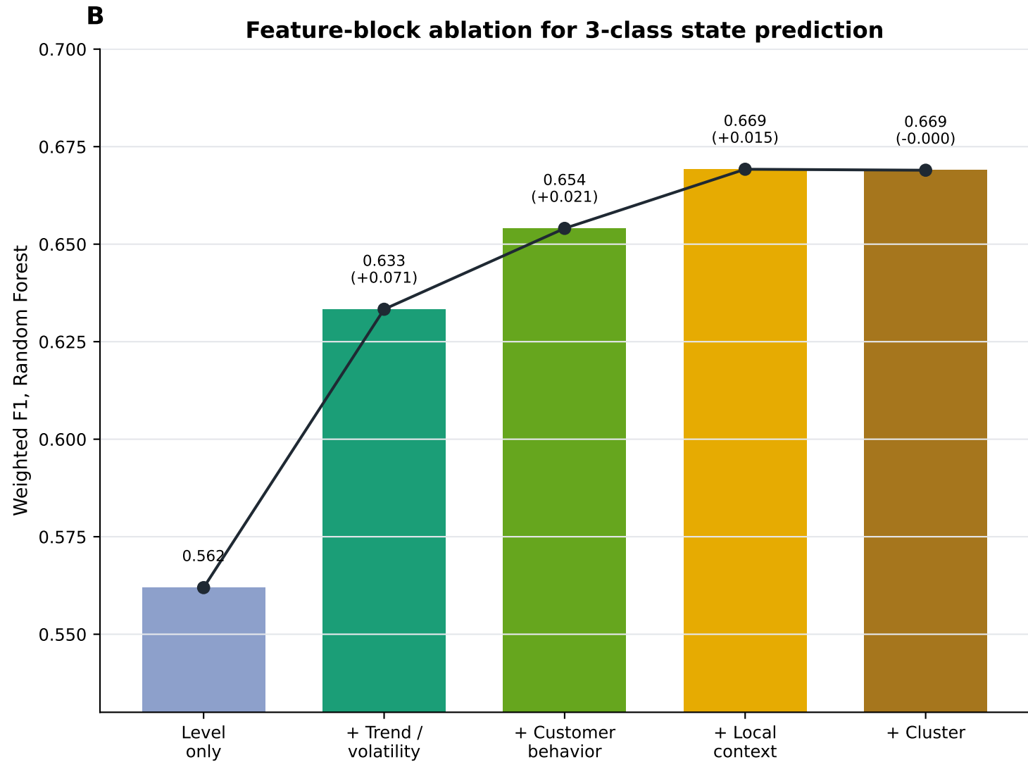
Figure 3. Early prediction improves with temporal dynamics and context
