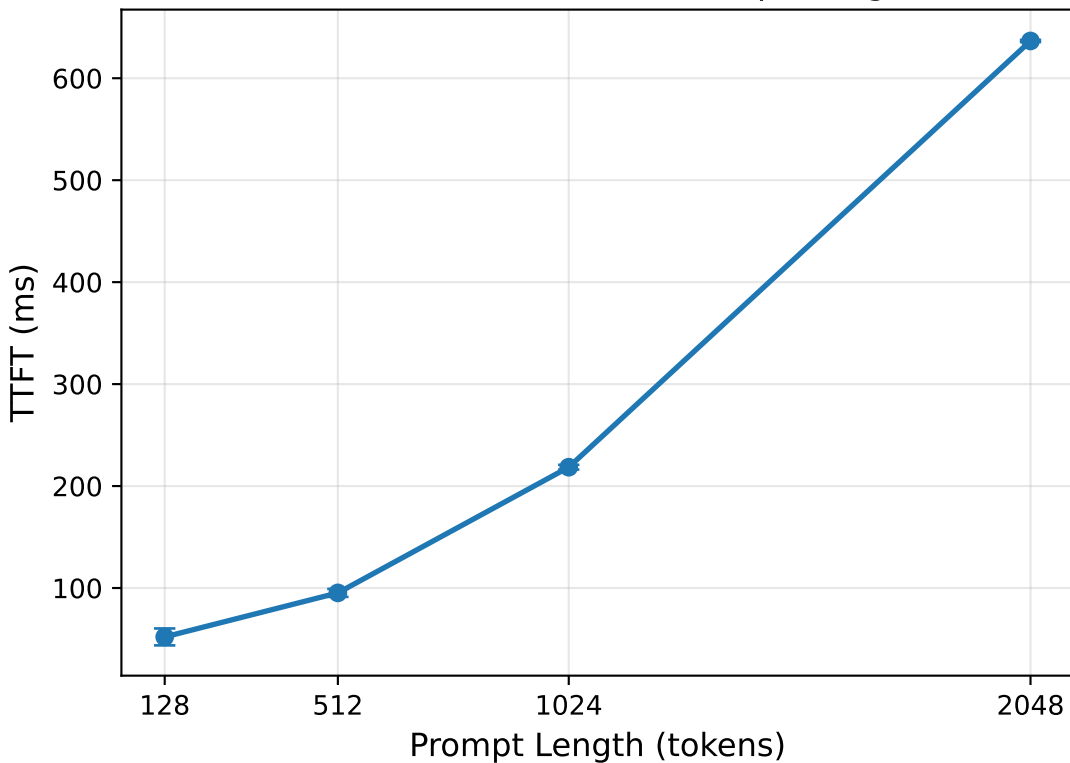
Time to First Token vs. Prompt Length
