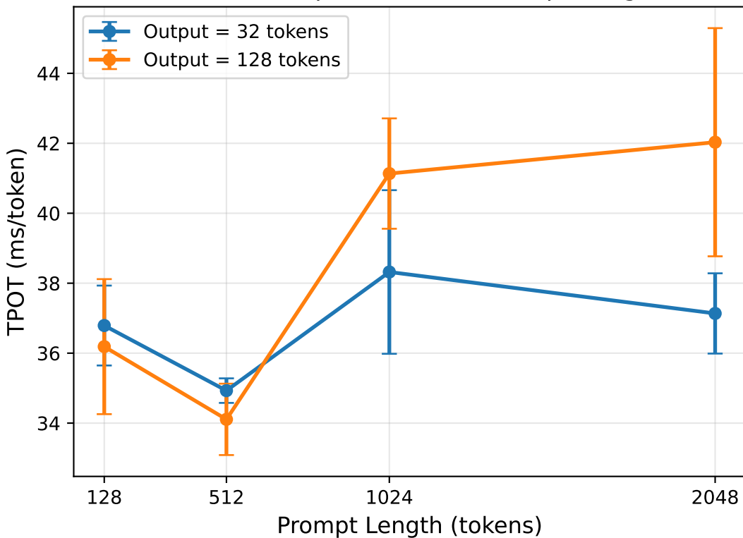
Time Per Output Token vs. Prompt Length
