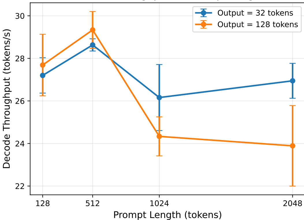
Decode Throughput vs. Prompt Length
