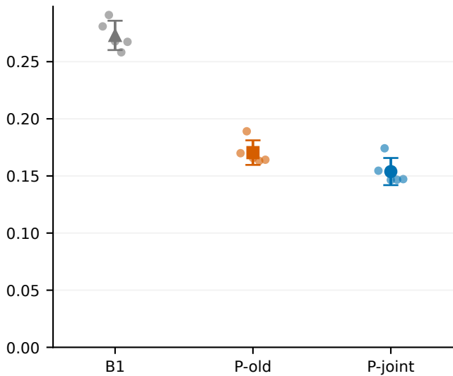
Multiclass log loss
