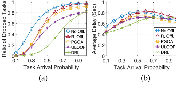
Fig. 5. Performance evaluation under different task arrival probabilities: (a) ratio of dropped tasks; (b) average delay.
