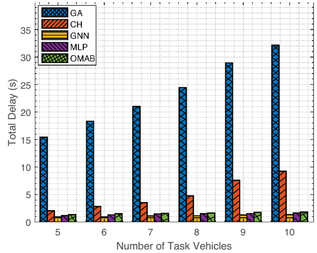
FIGURE 7 | Total delay with the increasing number of task vehicles.
