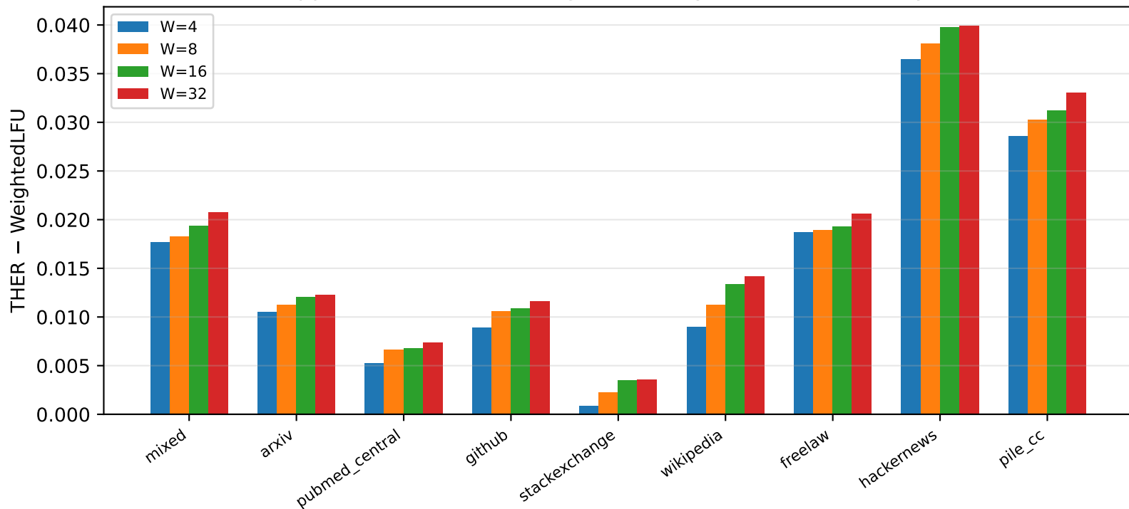
Supplemental: THER-WeightedLFU by domain (F=4, vary W)
