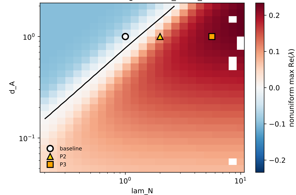
C. Phase diagram: \lambda_N \times d_A
