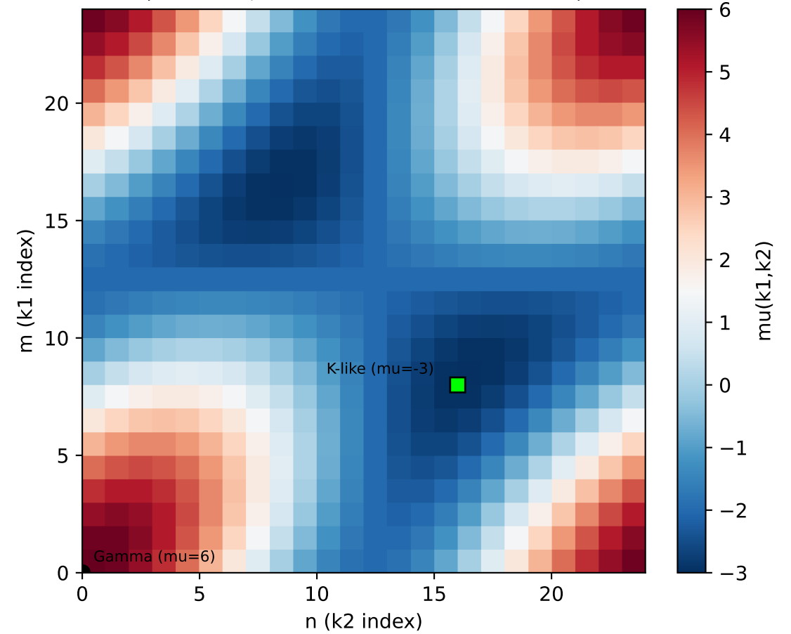
B. Graph dispersion \mu(k_1, k_2) (numerical, matches closed form to 2.8e-14 )
