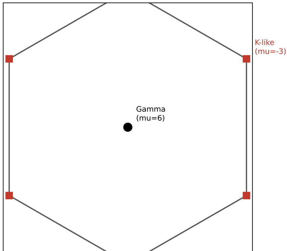
A. Brillouin zone of the triangular contact lattice (schematic)
