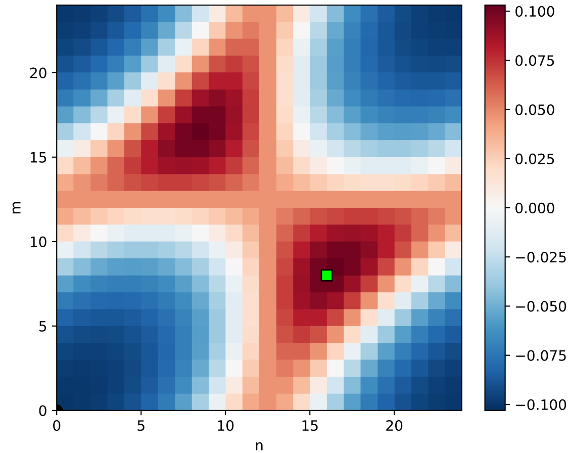
C. Growth-rate surface at \text{lam}_N=2.0 (P2) k=0 stable, K-like strongest growth
