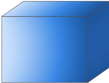
Label-free \delta = 0.202
