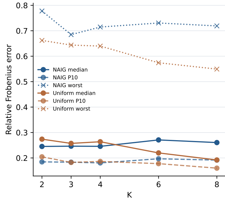
P4. Typical and lower-tail performance by K
