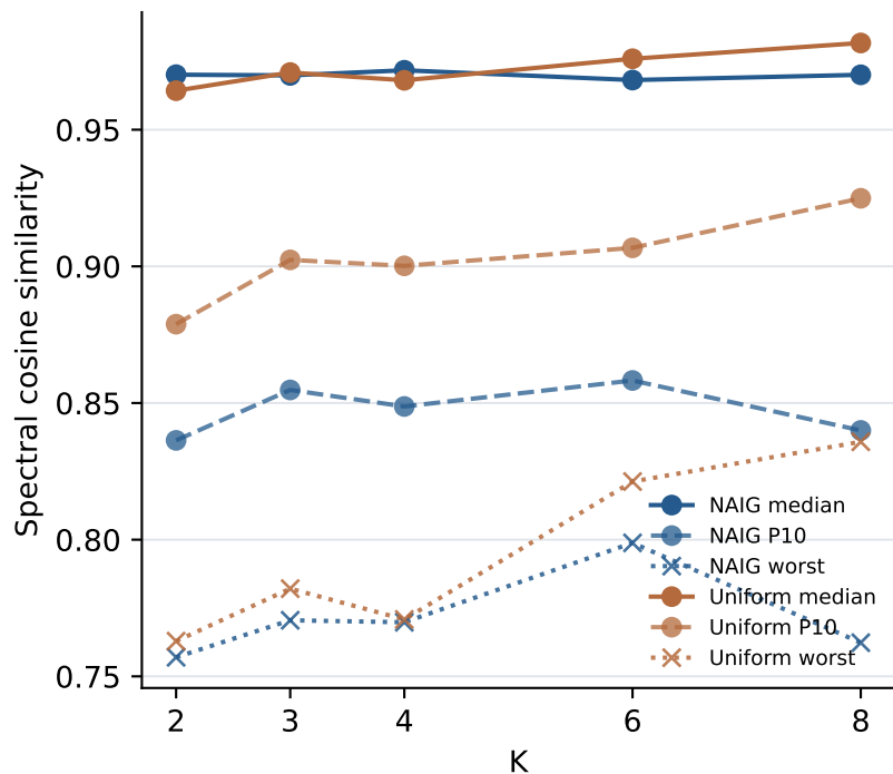
P4. Typical and lower-tail performance by K
