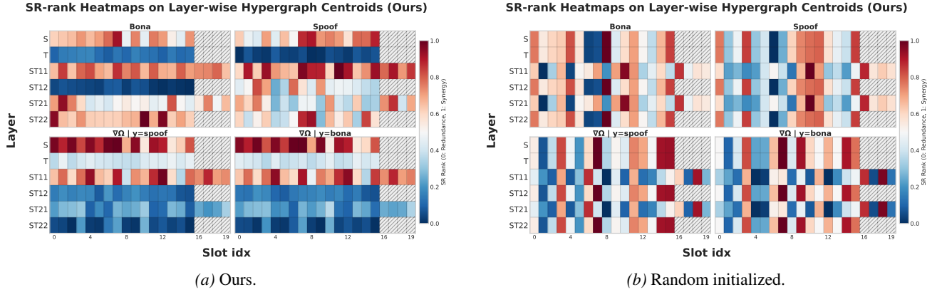
Figure 9. SR-rank heatmaps for global-prototype-aligned centroid slots across hypergraph layers: O-information ( \Omega ) and Gradient O-information conditioned on y ( \nabla\Omega \mid y ; y=\text{spoof} vs. y=\text{bona} ), with SR min-max normalized to [0, 1] (per panel), where 0 denotes redundancy-dominance and 1 denotes synergy-dominance.
