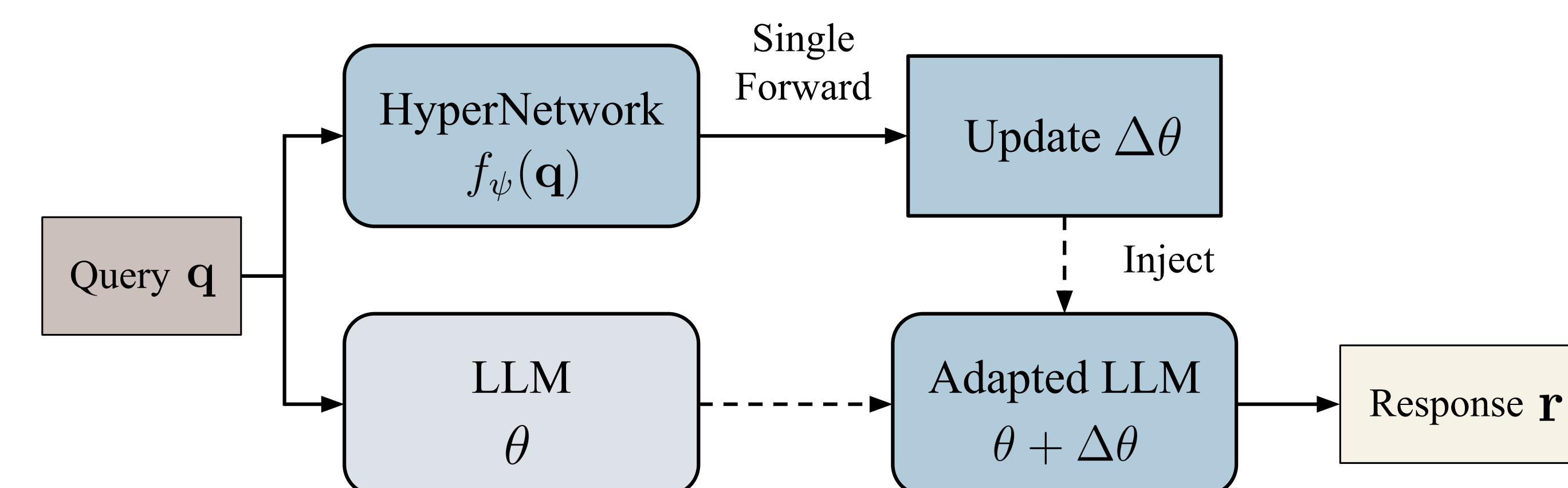
(c) HYPERTHINK (Ours)
