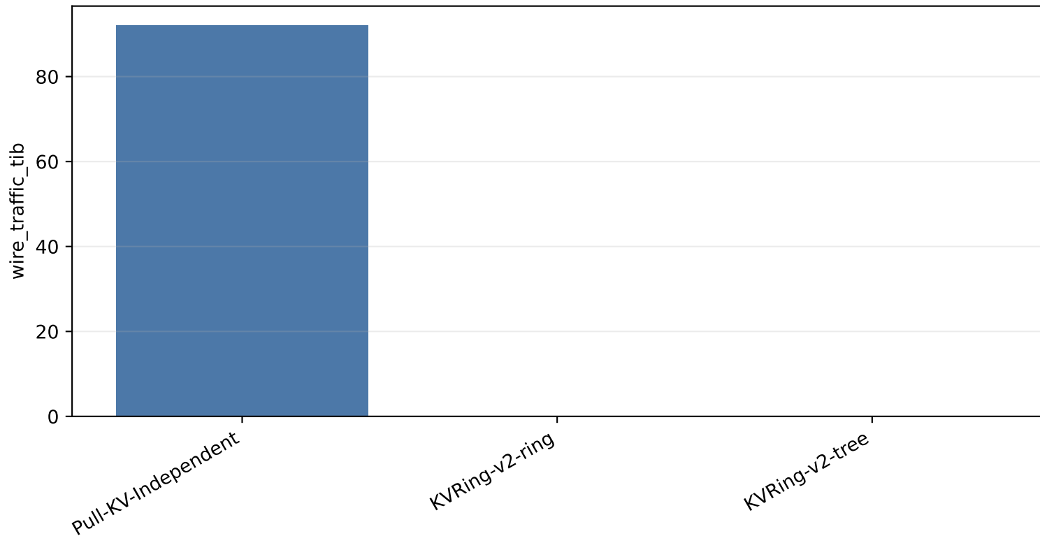
Moving KV vs Moving Query/States
