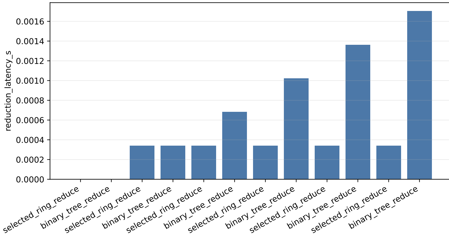
Ring vs Binary Tree Online-Softmax Reduction
