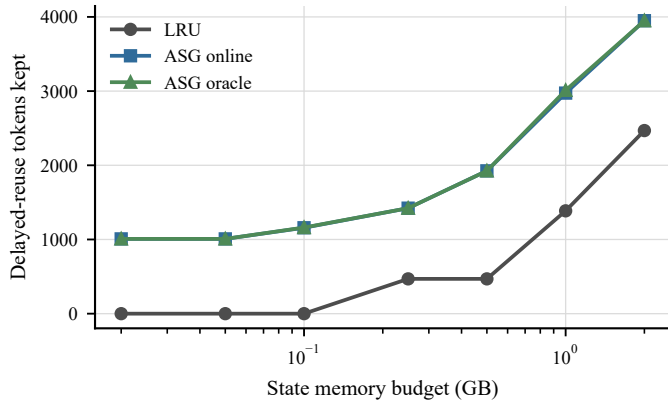
(a) Retention of LRU-regret state
