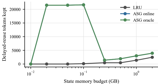
(c) LRU drops valuable delayed state
