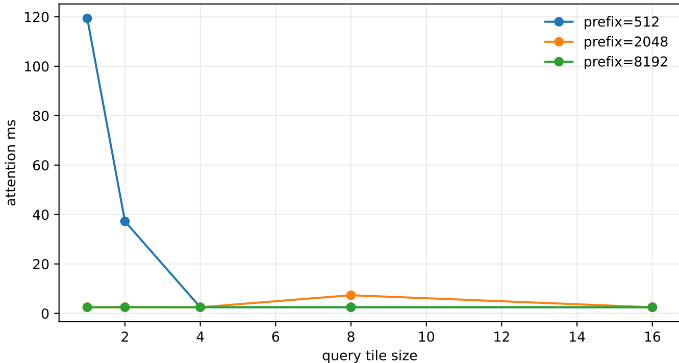
H100 Reduced Attention Microbench
