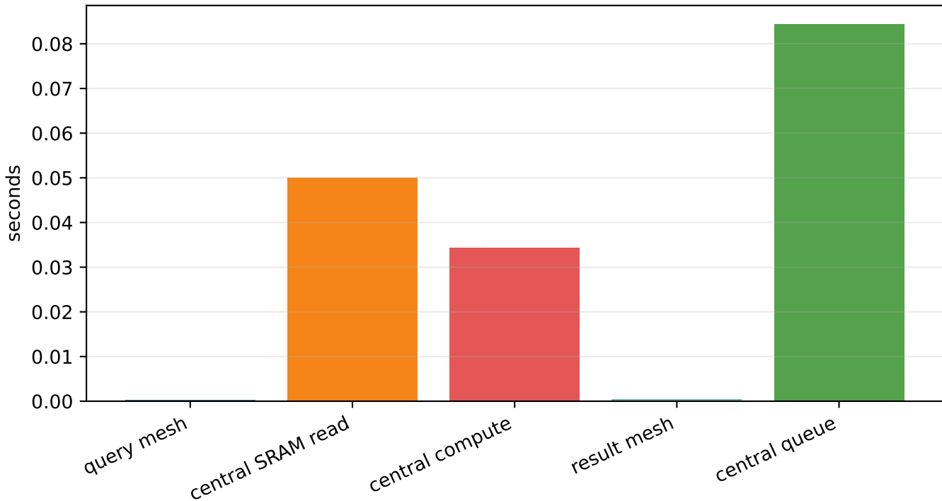
Central-KV-Stationary Bottleneck Breakdown
