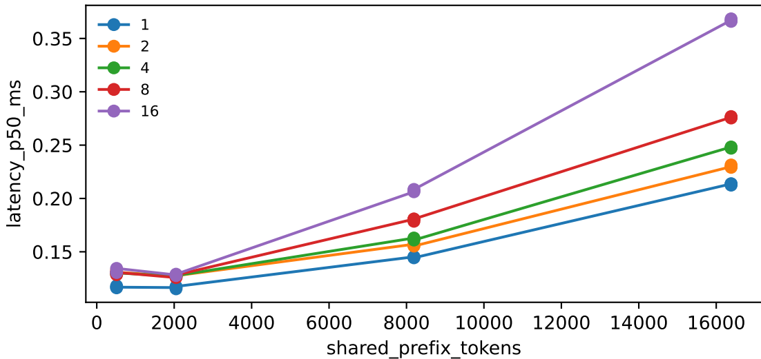
H100 microbench-fit shared-attention cost model
