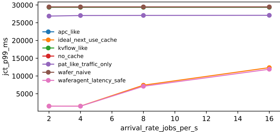
Trace-driven wafer simulation: p99 JCT
