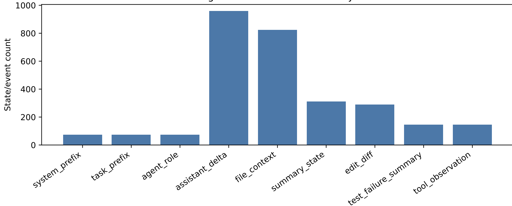
Agent Workflow State Anatomy
